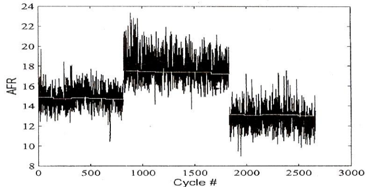
Figure 4. Estimated AFR (black line) and measured AFR (white line).
