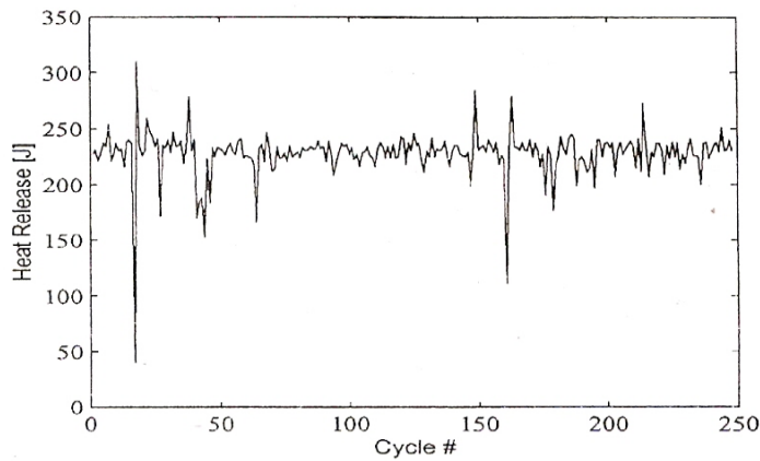
Fig.7. Heat release for 248 consecutive cycles at AFR = 18:1 . The plot clearly indicates incomplete combustion for several cycles. The estimated AFR for these cycles is 25.3.
