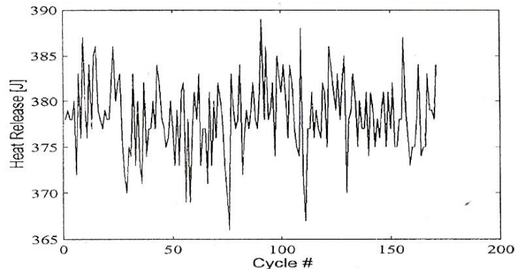
Figure 8. Heat release for 171 consecutive cycles at AFR = 14:76 : Compared to Figure-7 the heat release is almost constant from cycle to cycle, indicating that combustion is nearly complete.
