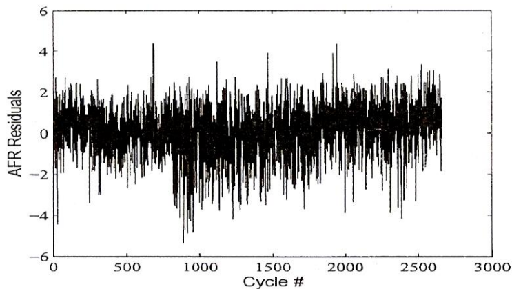
Figure5. Residuals of least-squares AFR fit.
