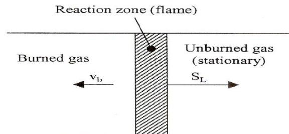
Figure 2. Illustration of a propagating laminar flame. The flame front moves at the Laminar flame speed, into the stationary unburned gas. Due to the expansion, the burned gas is pushed backwards out of the reaction zone at a velocity.
