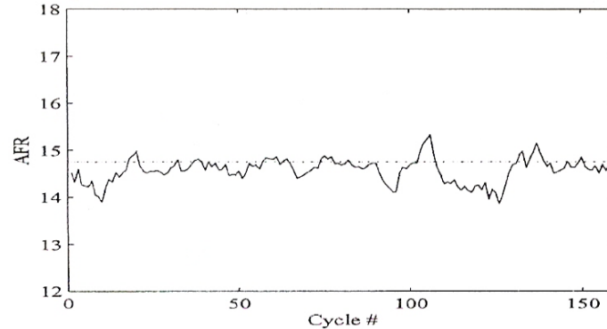
Figure. 9 Ten cycle moving average of AFR estimate. Steady-state operation with stoichiometric AFR.
