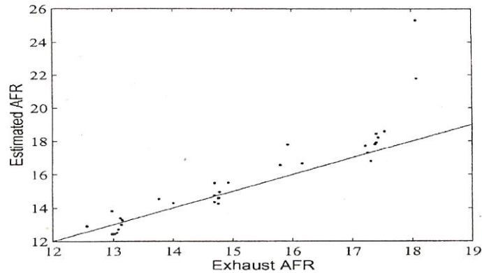
Fig.6. Cycle-averaged (10s) estimated AFR plotted versus measured exhaust AFR. Experiments conducted at a range of engine speeds, loads, and Air/Fuel Ratios. The RMS error in the estimate is 4% when excluding the two estimates at the lean limit ( AFR \geq 18 ).
