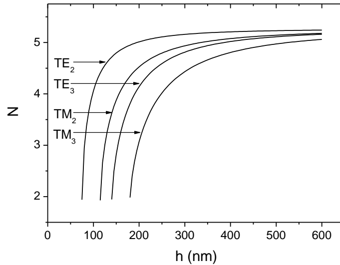
Figure 4. Comparison between TE and TM guided modes of silver-clad left-handed waveguide when \lambda = 632.8 \text{ nm} , \epsilon_c = 1 , \mu_c = 1 , \epsilon_g = -3.7+0.001i , \mu_g = -7.5+0.001i , \epsilon_m = -16+0.52i , and \mu_m = 1 .
