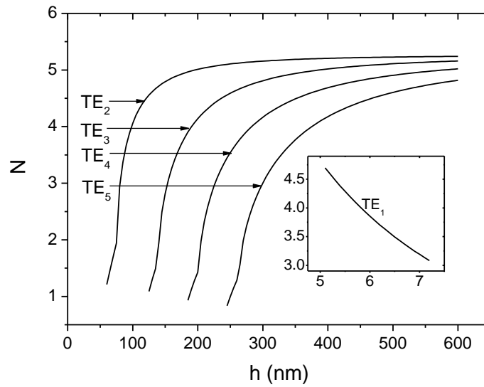
Figure 2. The modal index for TE guided modes of silver-clad left-handed waveguide when \lambda = 632.8 nm, \epsilon_c = 1 , \mu_c = 1 , \epsilon_g = -3.7+0.001i , \mu_g = -7.5+0.001i , \epsilon_m = -16+0.52i , and \mu_m = 1 .
