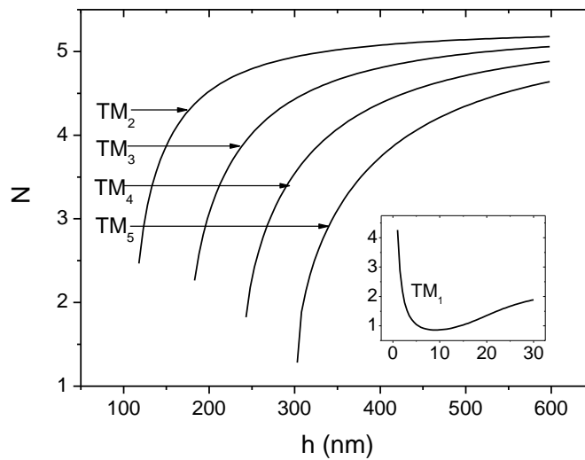
Figure 3. The modal index for TM guided modes of silver-clad left-handed waveguide when \lambda = 632.8 nm, \epsilon_c = 1 , \mu_c = 1 , \epsilon_g = -3.7+0.001i , \mu_g = -7.5+0.001i , \epsilon_m = -16+0.52i , and \mu_m = 1 .
